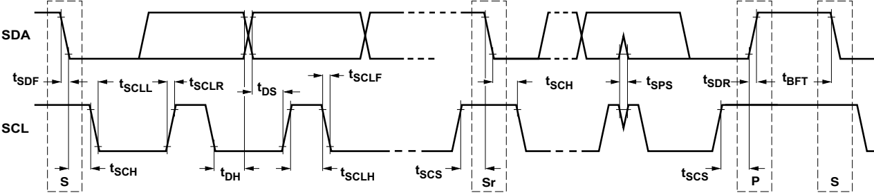
Figure 10. I 2 C Port Timing
