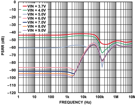
Figure 7. VOUT2 PSRR, I_{\text{VOUT2}} = 10 \text{ mA}
