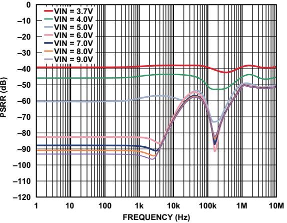
Figure 8. VOUT2 PSRR, I_{\text{VOUT2}} = 50 \text{ mA}
