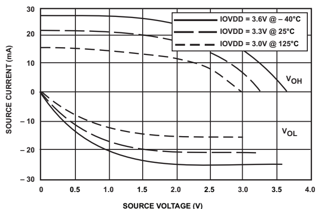
Figure 22. Digital I/O Drivers (DS0, 3.3 V IOVDD)
