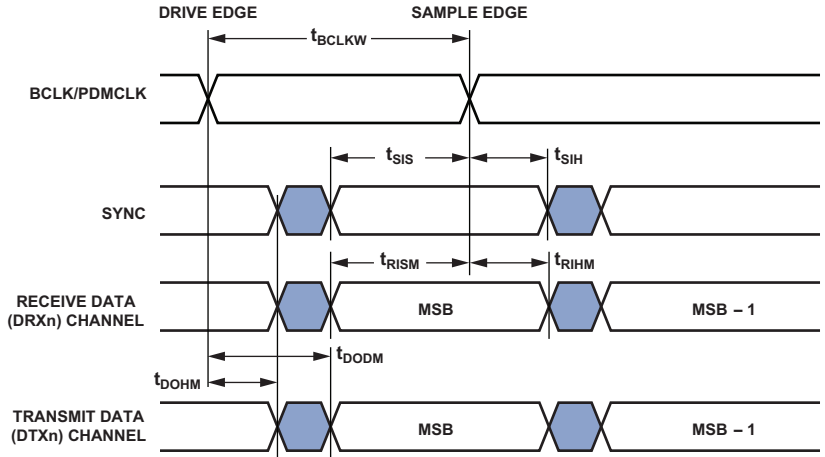
Figure 11. I 2 S Slave (A 2 B Main Node) Timing
