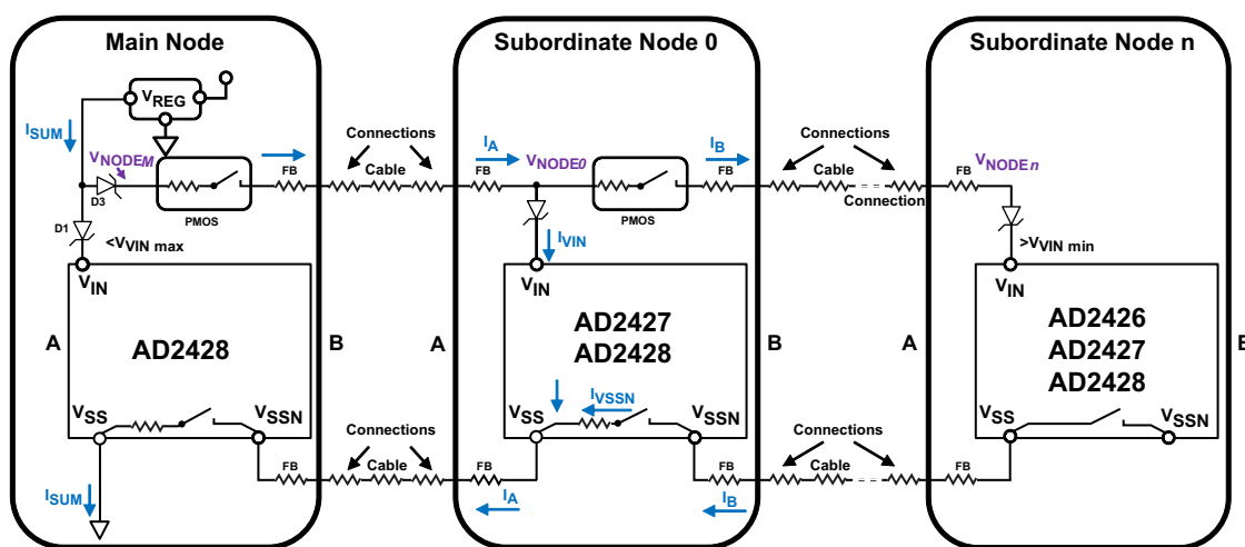
Figure 37. A 2 B Power Model for Bus Powered System
