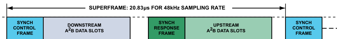
Figure 3. A 2 B Superframe
