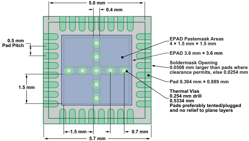
Figure 39. Transceiver Footprint
