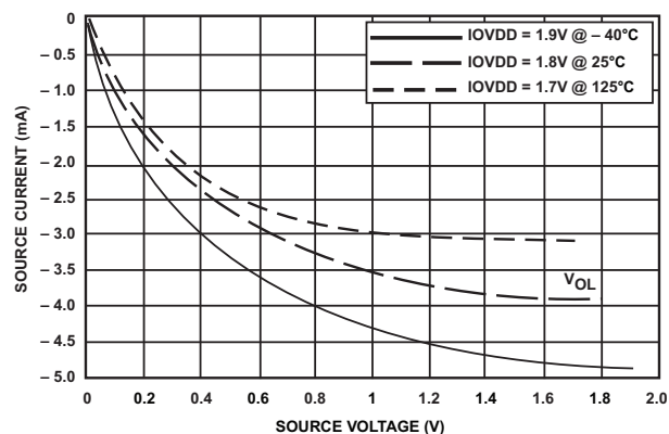
Figure 23. I 2 C Drivers (1.8 V IOVDD)
