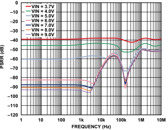
Figure 8. VOUT2 PSRR, I_{\text{OUT2}} = 50 \text{ mA}
