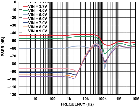
Figure 7. VOUT2 PSRR, I_{\text{OUT2}} = 10 \text{ mA}
