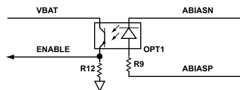
Figure 38. Optional Power Supply Enable Circuit with Optocoupler
