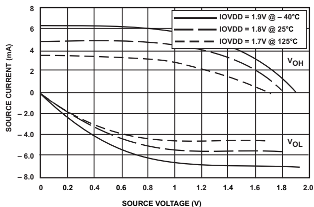
Figure 21. Digital I/O Drivers (DS0, 1.8 V IOVDD)
