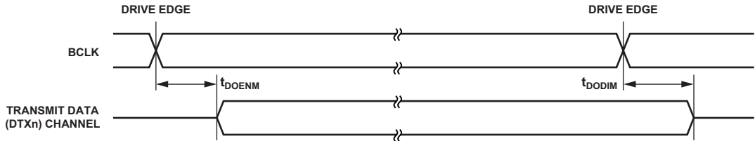
Figure 13. I 2 S Slave (A 2 B Main Node) Enable and Three-State Timing
